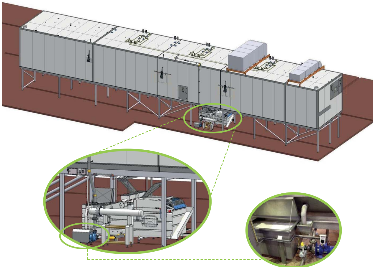
CIP retourtank 500L
